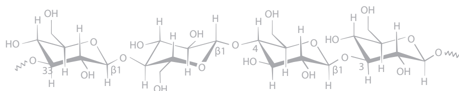
The chemical structure of oat beta-glucan molecule.
